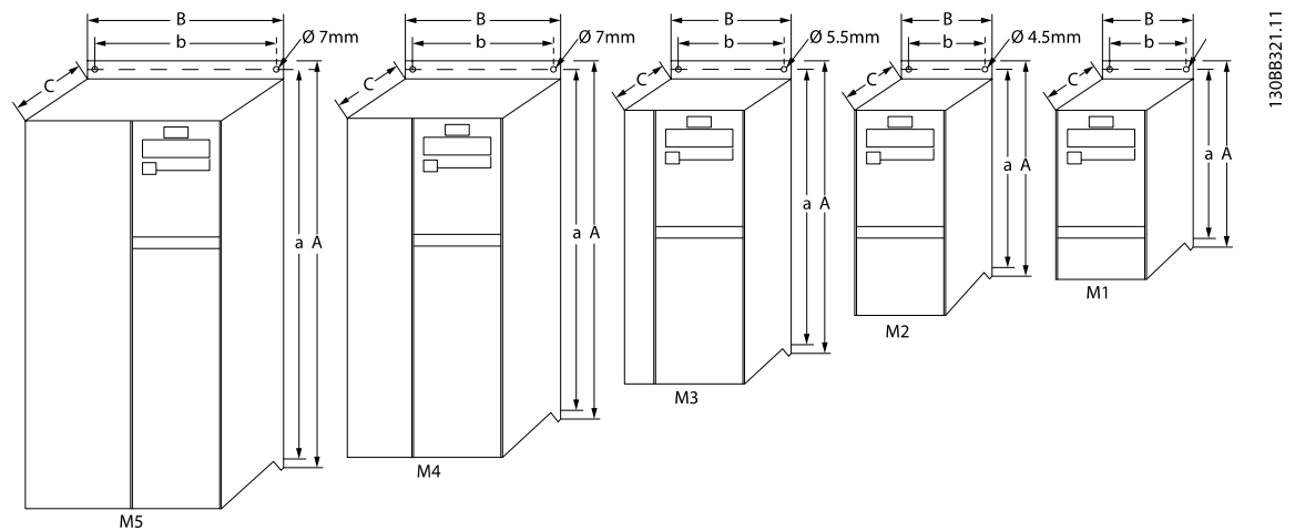
Illustration 1.1: Mechanical dimensions.
